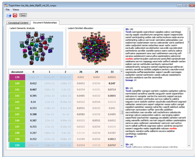
Figure 2: For the alphabet data set, the Document Table and Document Text views in the Document Relationships panel show that LSA concept 0 contains only “o” documents (140-149), whereas LDA topic 33 has a mixed set of weights for that cluster.
