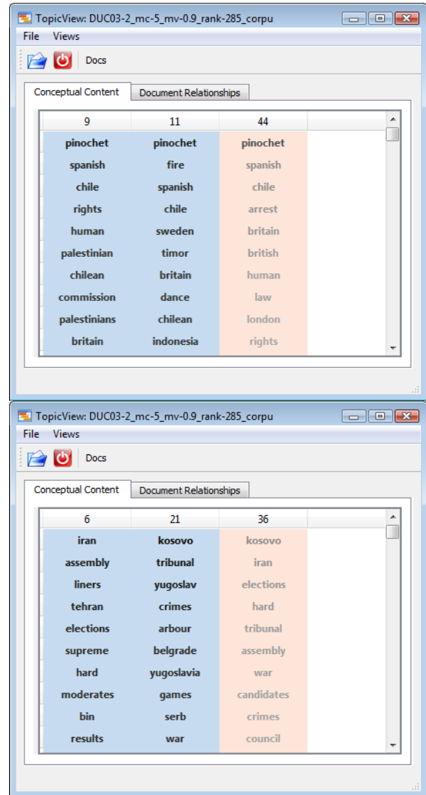
Figure 7: Top 10 terms associated with the concepts/topics where multiple LSA concepts are strongly connected to a single LDA topic.
