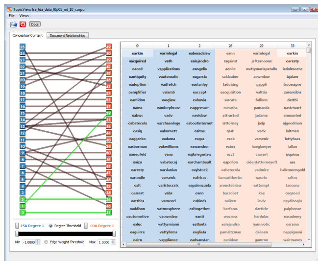
Figure 1: Relationships between LSA concepts (blue) and LDA topics (red) for the alphabet data set. The LSA concepts identify the independent term sets in the data, whereas terms starting with different letters are highly mixed across LDA topics.
