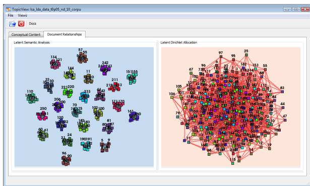
Figure 3: Graphs depicting document relationships modeled using LSA (left) and LDA (right) for the alphabet data set.
