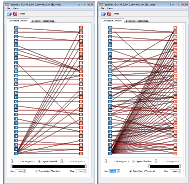
Figure 6: Graphs depicting conceptual content relationships for the DUC data set modeled with LSA (blue nodes) and LDA (red nodes) using a minimum degree threshold of 1 for LSA/LDA nodes (left) and a minimum edge threshold of 0.1760 (right).
