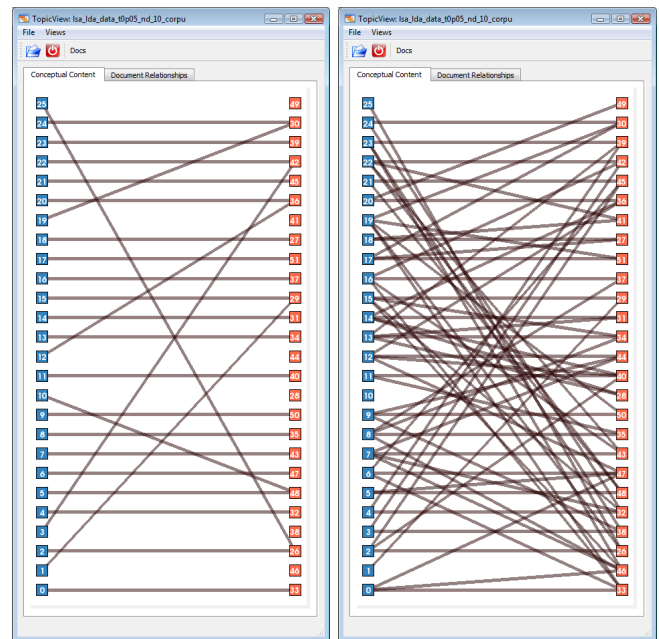
Figure 4: Graphs depicting conceptual contents relationships for the alphabet data set modeled with LSA (blue nodes) and LDA (red nodes) using a minimum degree threshold of 1 for LSA concept nodes (left) and a minimum edge threshold of 0.1451 (right).
